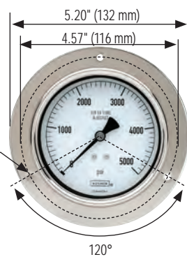
40-400/500 Rear Flange
