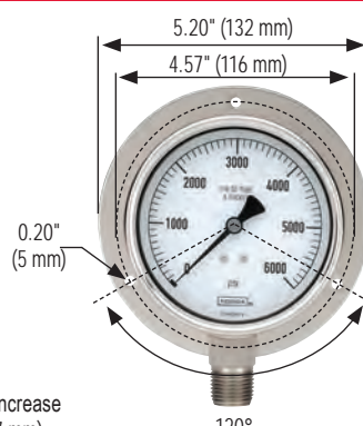
40-400/500 Rear Flange
