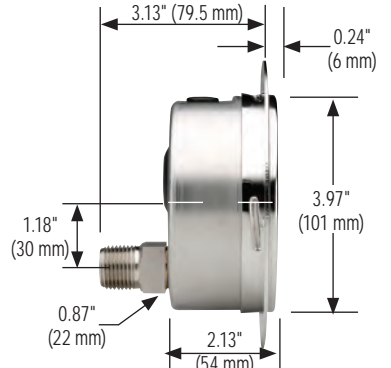
40-400/500 Rear Flange
