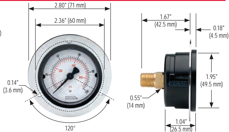
20-110 Front Flange
