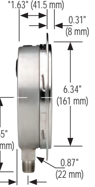
60-400/500 Front Flange
