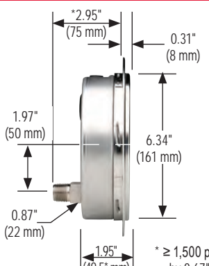
60-410/510 Front Flange
