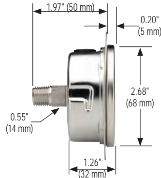
60-410/510 Front Flange
