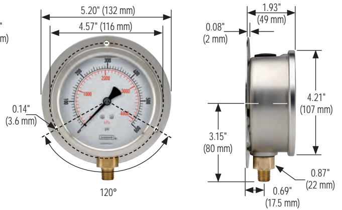
40-901 Rear Flange
