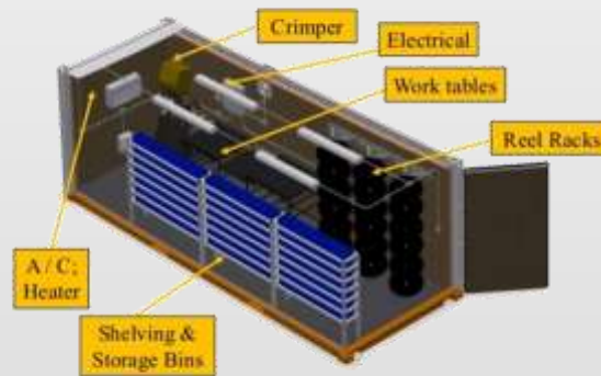
Sample Layout
